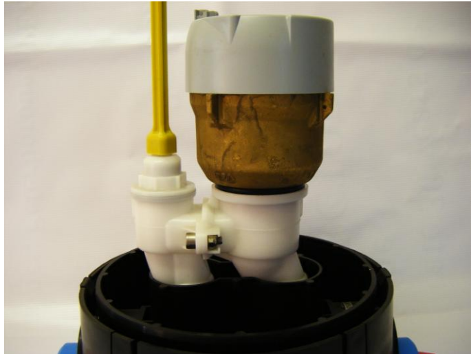
Side view with meter screwed into manifold
